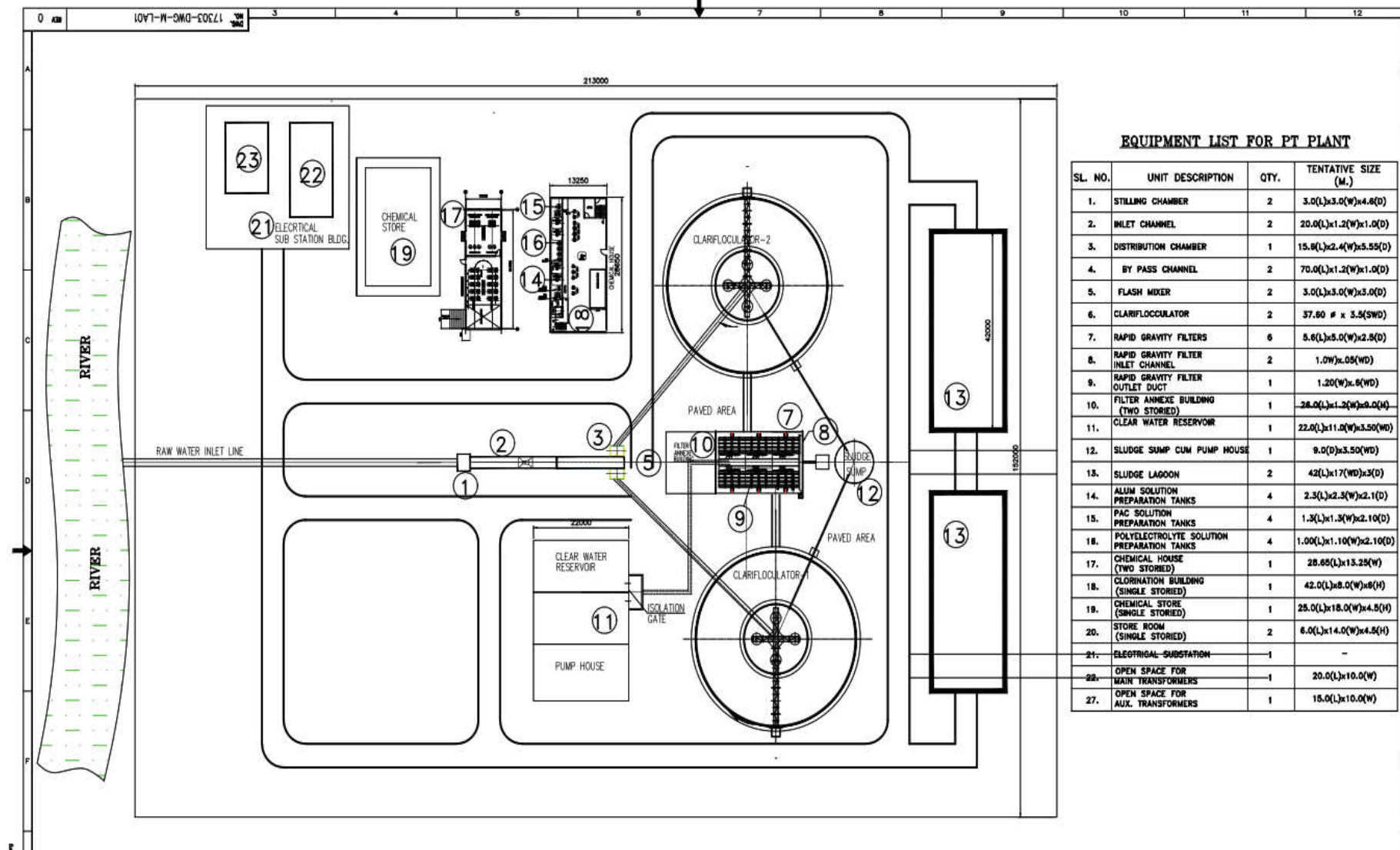
Figure 6: Layout Diagram of Proposed Water Treatment Plan
